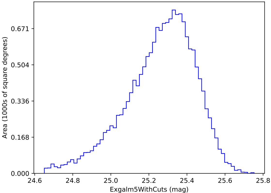
ddf_loaded_fl15_v3.4_10yrs i band non-DD year 1: ExgalM5WithCuts
