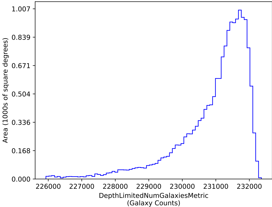
ddf_loaded_fl15_v3.4_10yrs i band galaxies non-DD: DepthLimitedNumGalaxiesMetric
