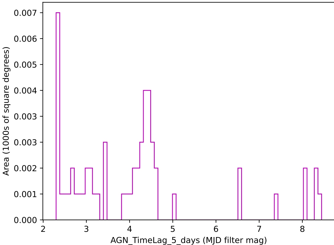
ddf_loaded_fl15_v3.4_10yrs z band: AGN_TimeLag_5_days
