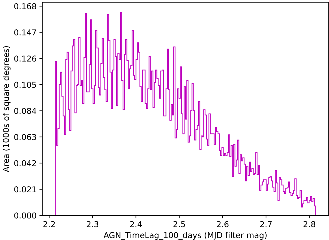
ddf_loaded_fl15_v3.4_10yrs z band: AGN_TimeLag_100_days
