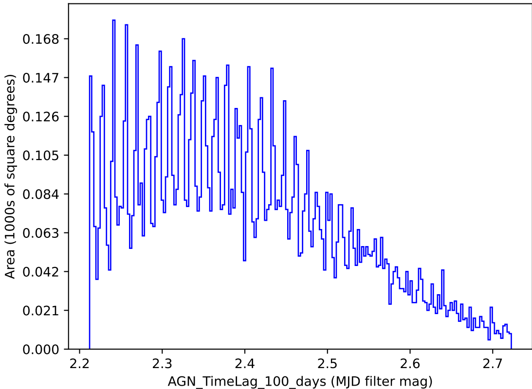
ddf_loaded_fl15_v3.4_10yrs y band: AGN_TimeLag_100_days
