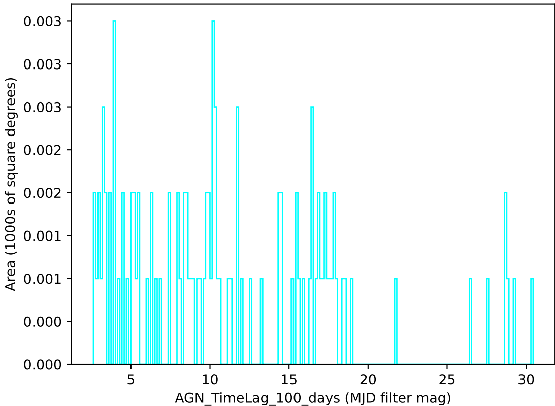
ddf_loaded_fl15_v3.4_10yrs u band: AGN_TimeLag_100_days
