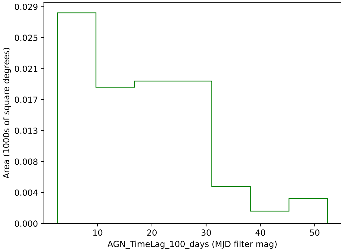
ddf_loaded_fl15_v3.4_10yrs g band: AGN_TimeLag_100_days
