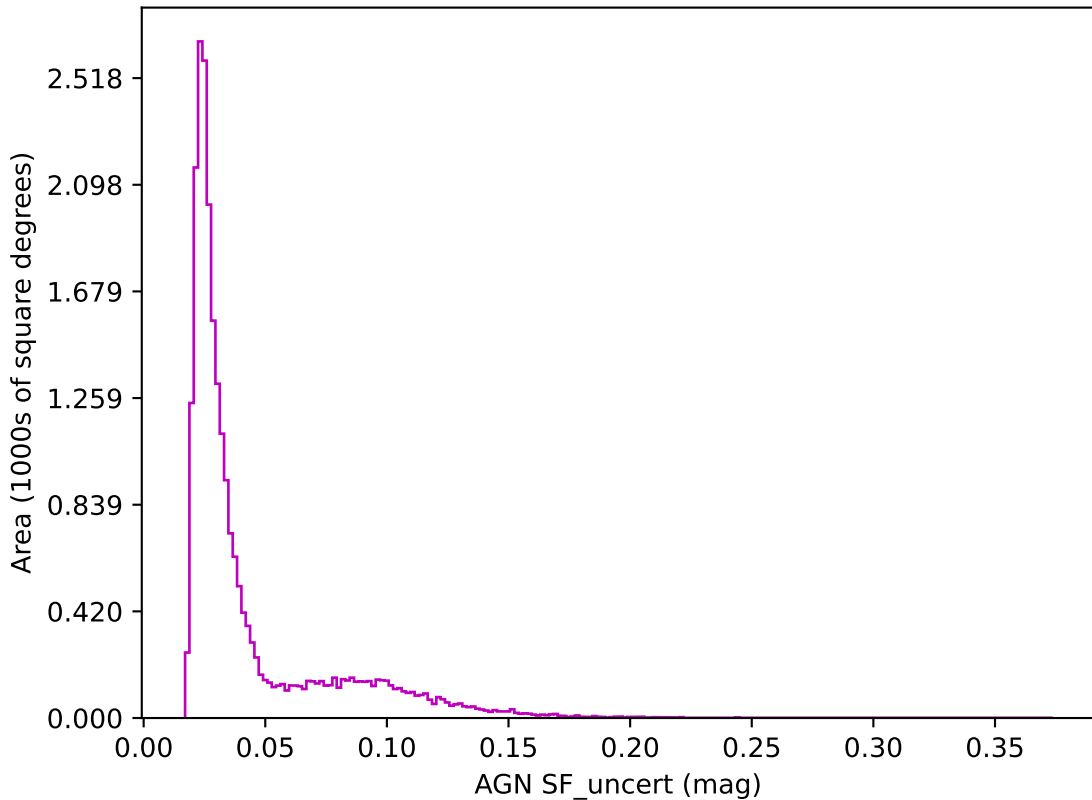
ddf_loaded_fl15_v3.4_10yrs z band: AGN SF_uncert
