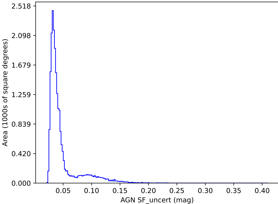
ddf_loaded_fl15_v3.4_10yrs y band: AGN SF_uncert
