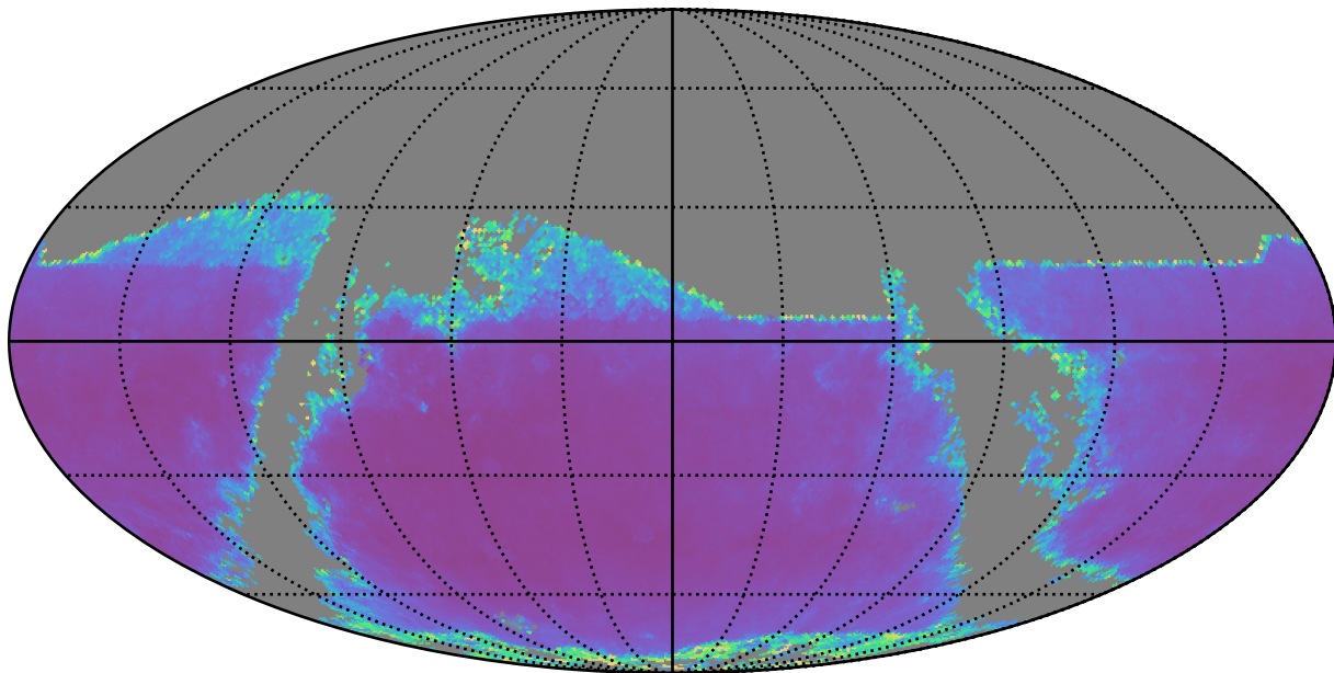
ddf_loaded_fl15_v3.4_10yrs r band: AGN SF_uncert
