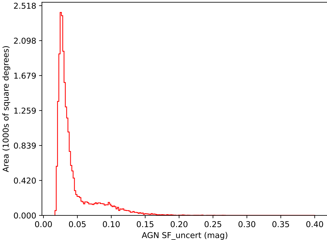
ddf_loaded_fl15_v3.4_10yrs i band: AGN SF_uncert
