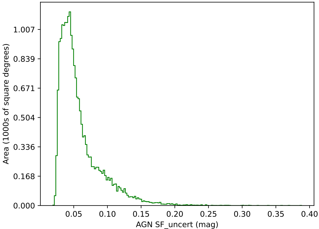
ddf_loaded_fl15_v3.4_10yrs g band: AGN SF_uncert
