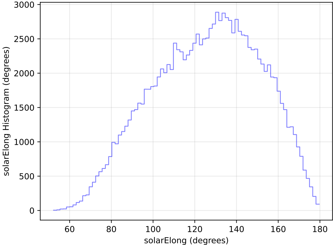
ddf_loaded_fl15_v3.4_10yrs WFD u band: solarElong Histogram
