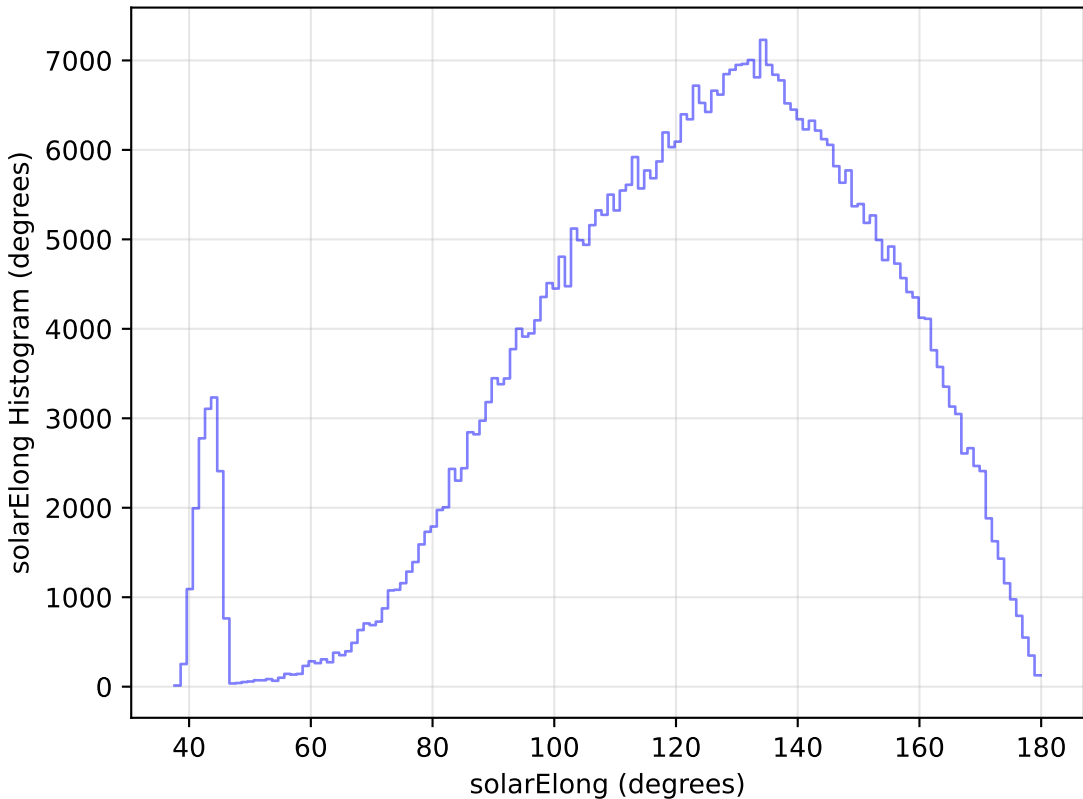
ddf_loaded_fl15_v3.4_10yrs WFD r band: solarElong Histogram
