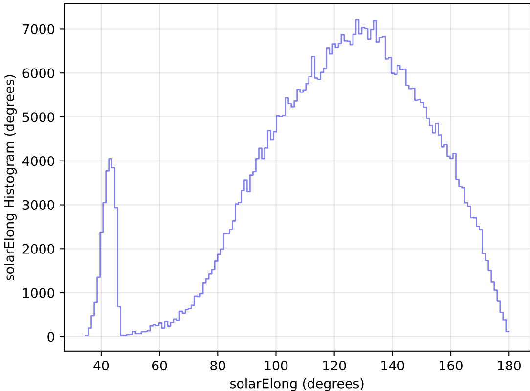
ddf_loaded_fl15_v3.4_10yrs WFD i band: solarElong Histogram
