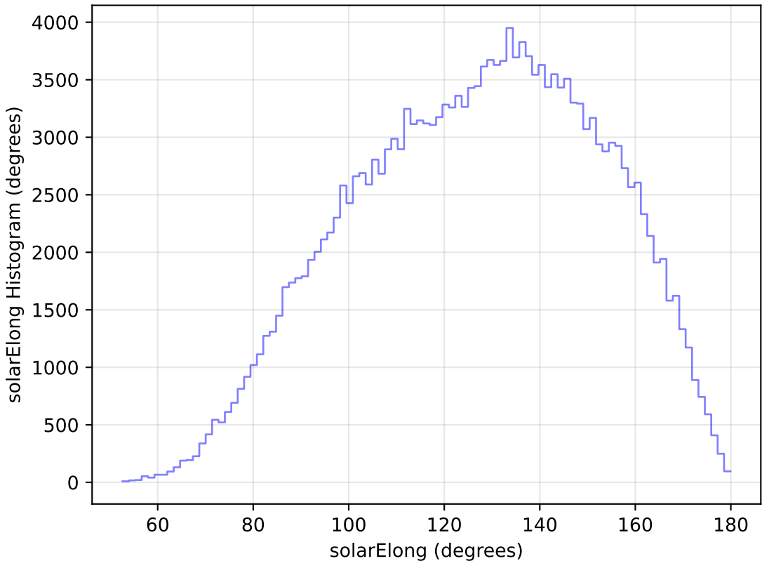
ddf_loaded_fl15_v3.4_10yrs WFD g band: solarElong Histogram
