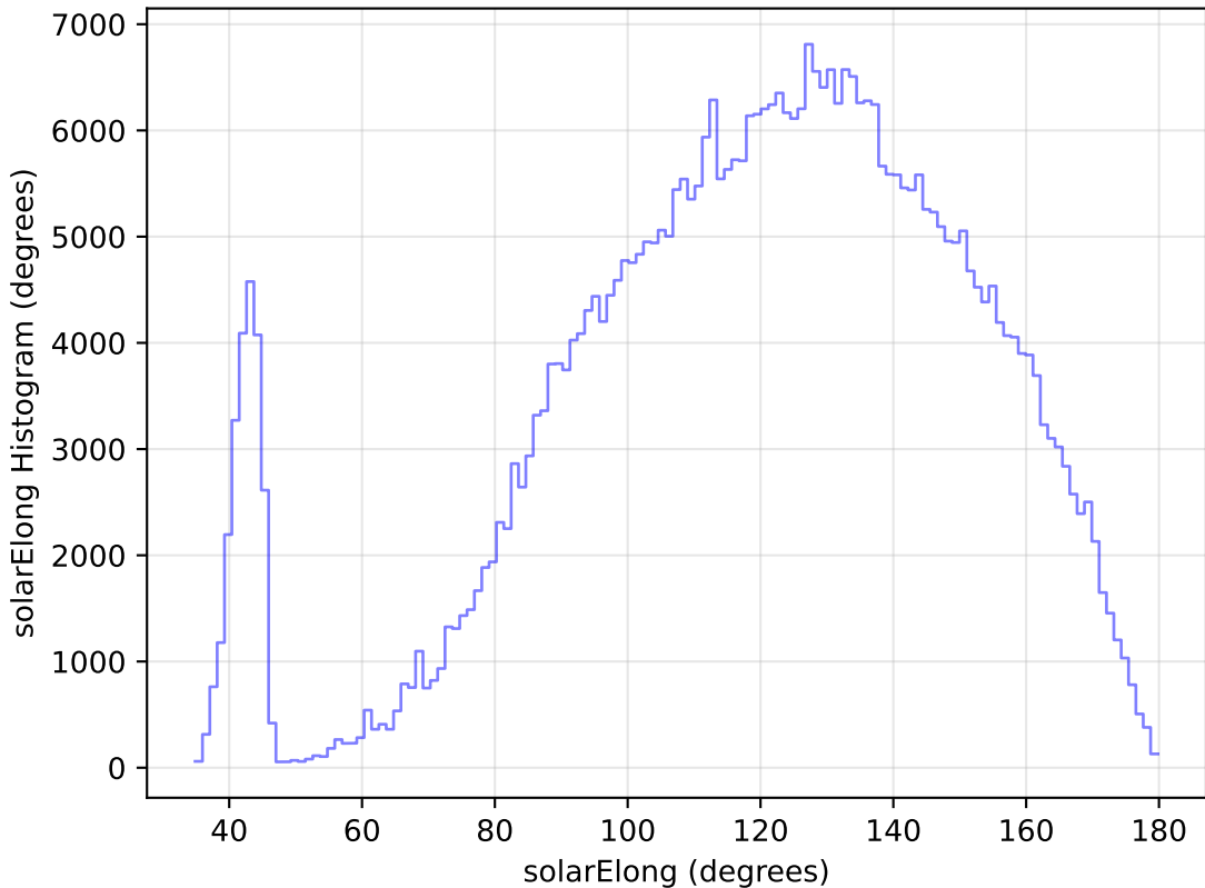
ddf_loaded_fl15_v3.4_10yrs All sky z band: solarElong Histogram
