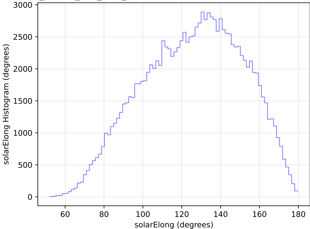
ddf_loaded_fl15_v3.4_10yrs All sky u band: solarElong Histogram
