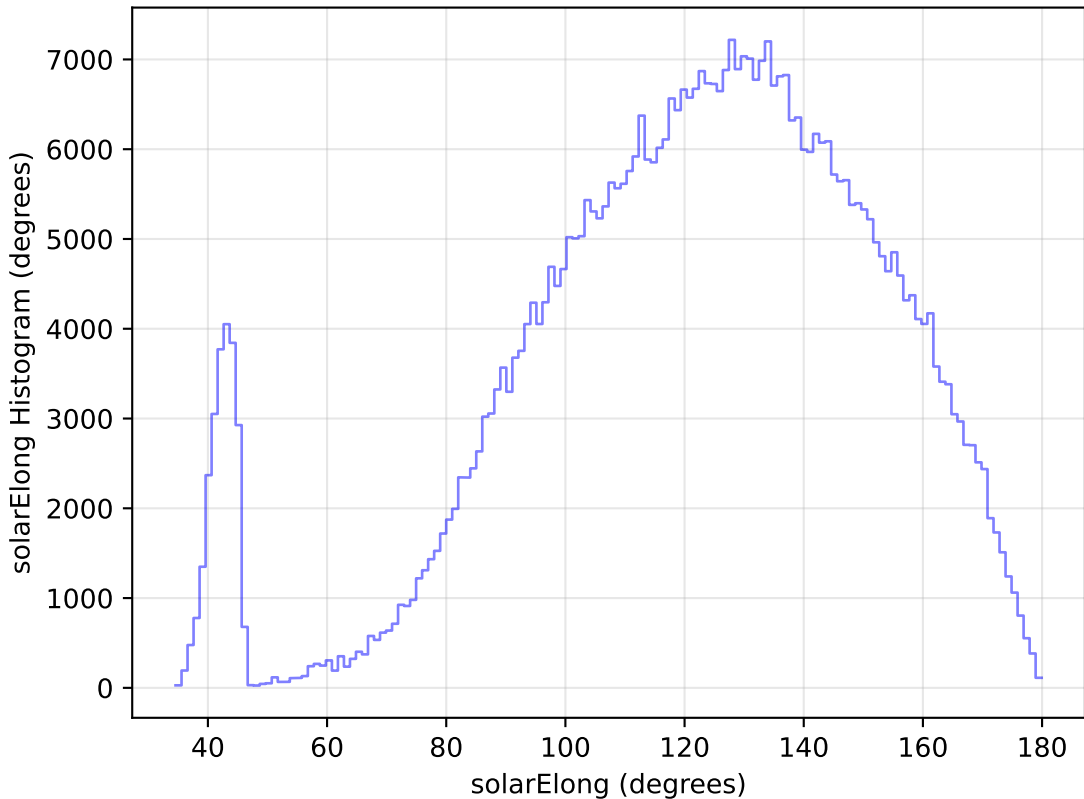
ddf_loaded_fl15_v3.4_10yrs All sky i band: solarElong Histogram
