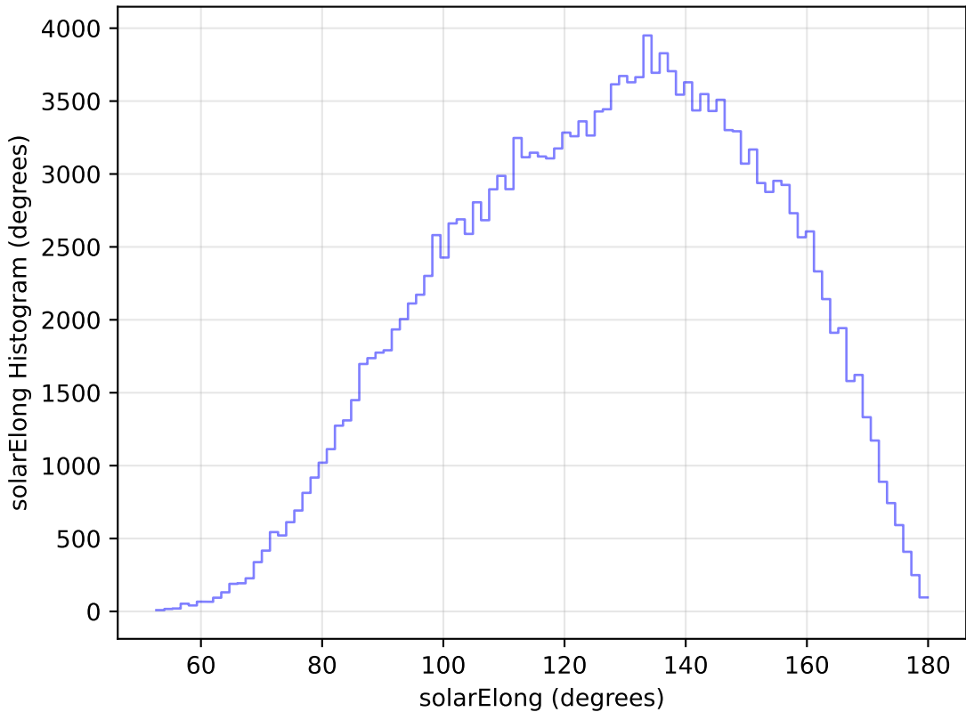
ddf_loaded_fl15_v3.4_10yrs All sky g band: solarElong Histogram
