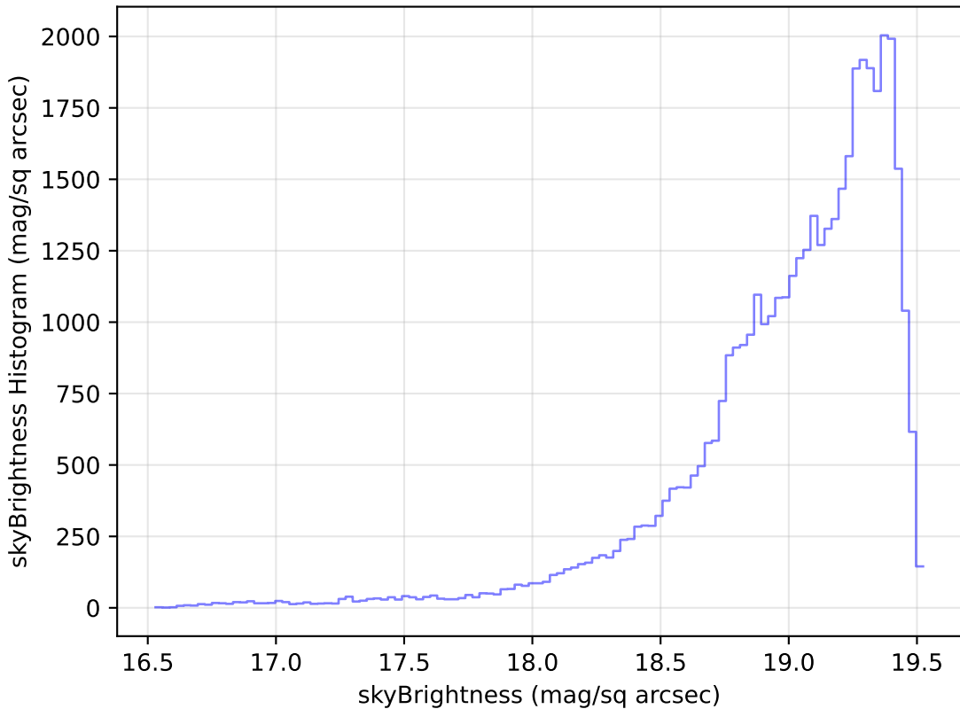
ddf_loaded_fl15_v3.4_10yrs Yr 1 z band: skyBrightness Histogram
