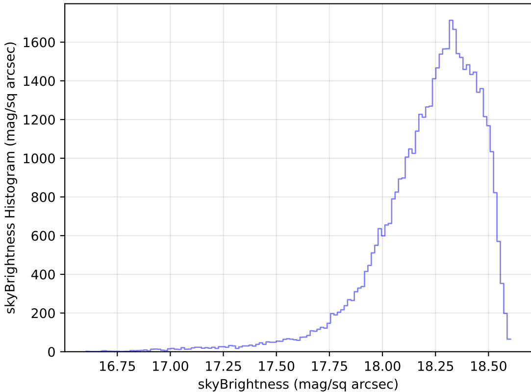
ddf_loaded_fl15_v3.4_10yrs Yr 1 y band: skyBrightness Histogram
