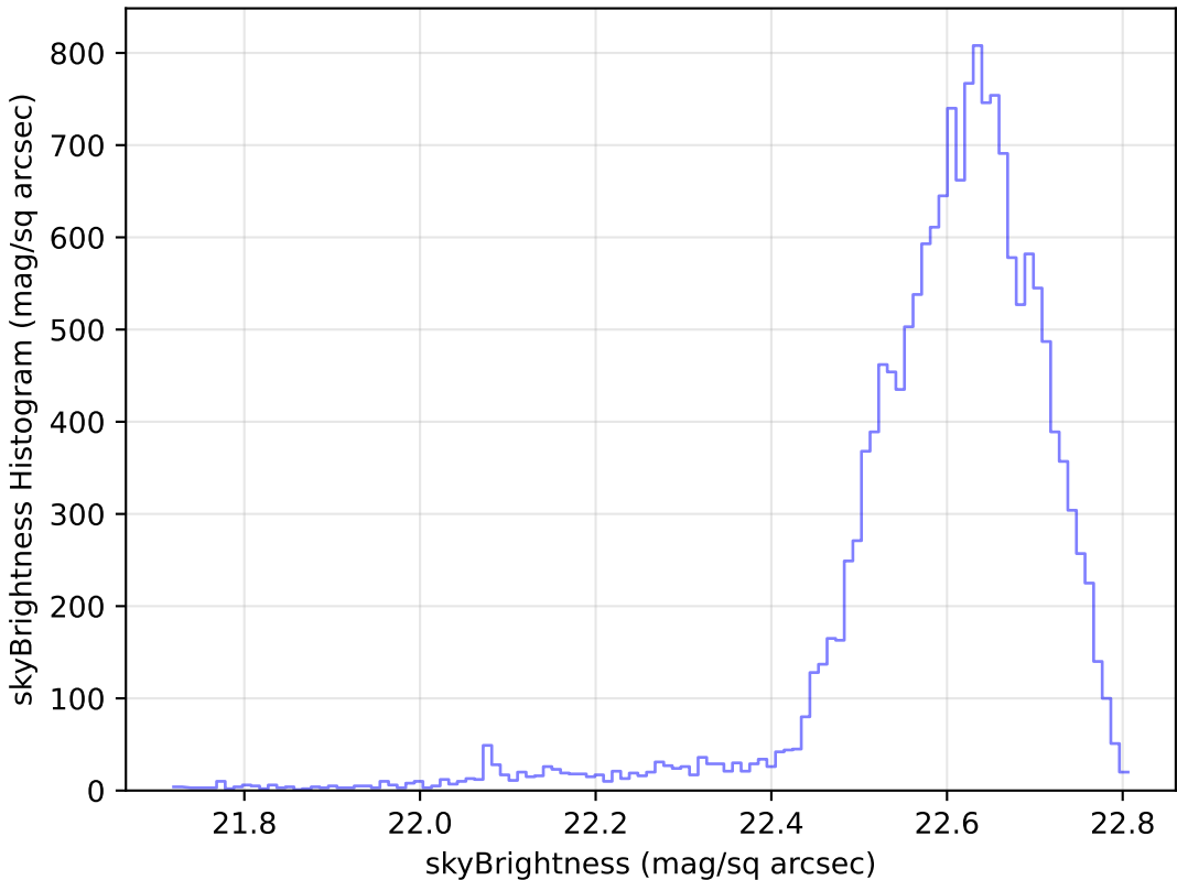
ddf_loaded_fl15_v3.4_10yrs Yr 1 u band: skyBrightness Histogram
