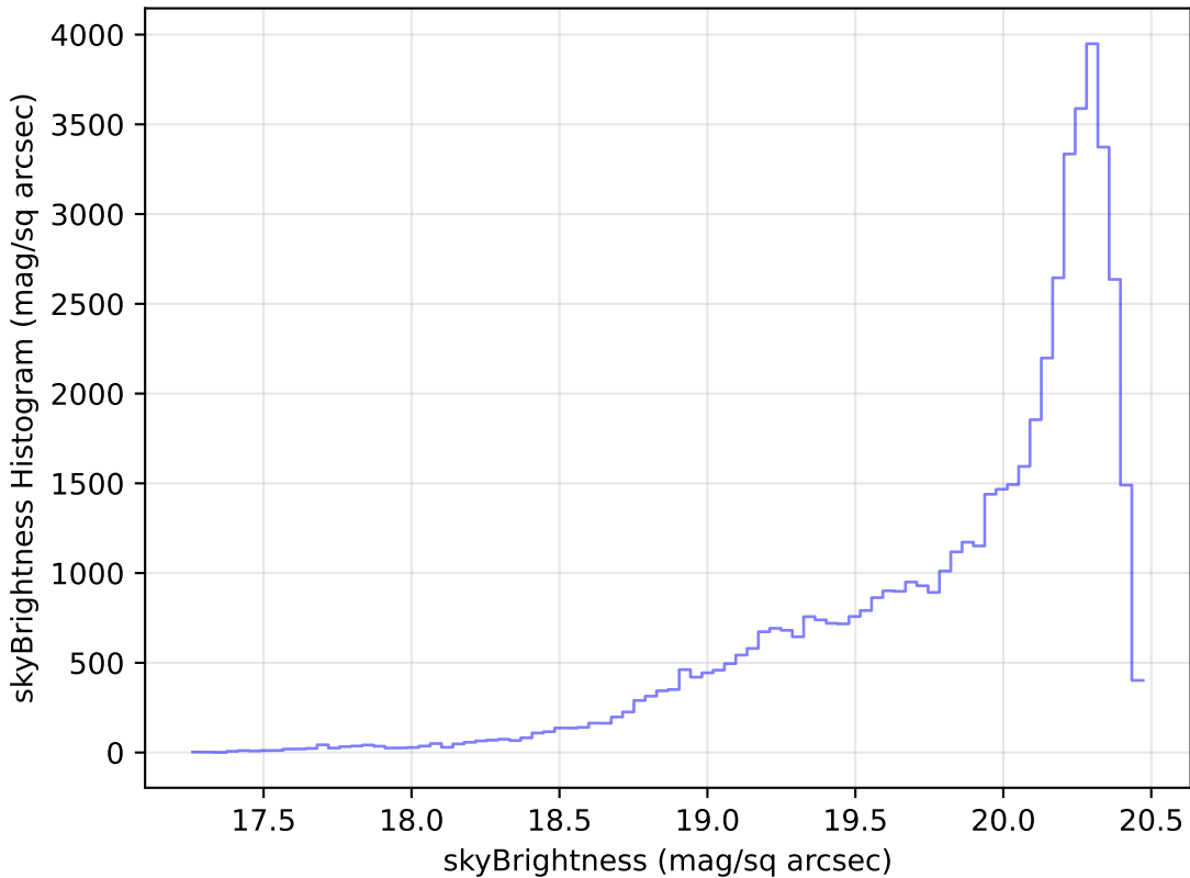
ddf_loaded_fl15_v3.4_10yrs Yr 1 i band: skyBrightness Histogram
