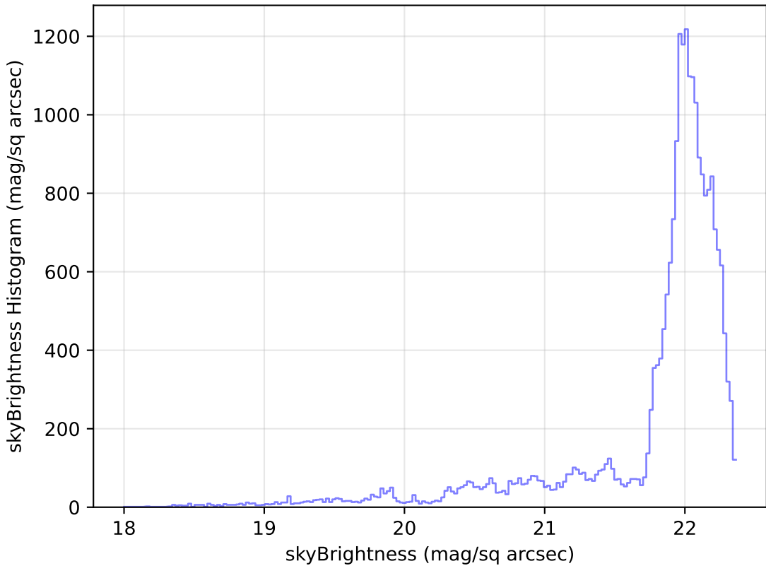
ddf_loaded_fl15_v3.4_10yrs Yr 1 g band: skyBrightness Histogram
