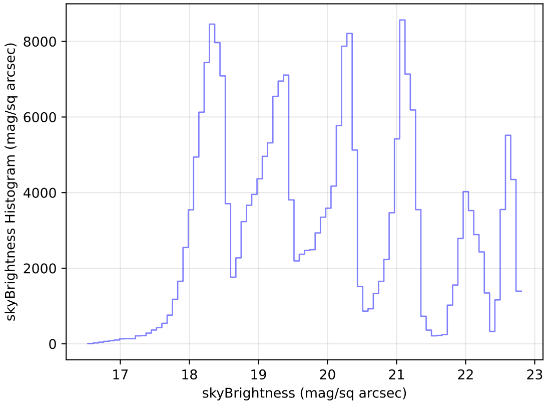
ddf_loaded_fl15_v3.4_10yrs Yr 1 all bands: skyBrightness Histogram
