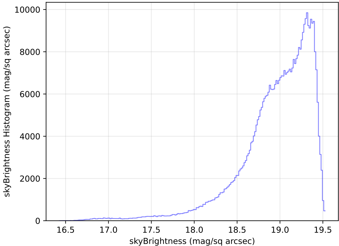
ddf_loaded_fl15_v3.4_10yrs WFD z band: skyBrightness Histogram
