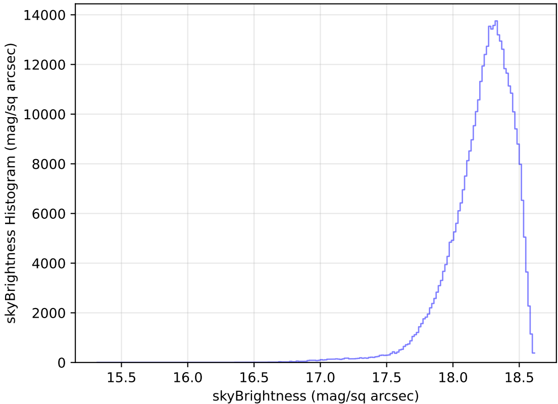
ddf_loaded_fl15_v3.4_10yrs WFD y band: skyBrightness Histogram
