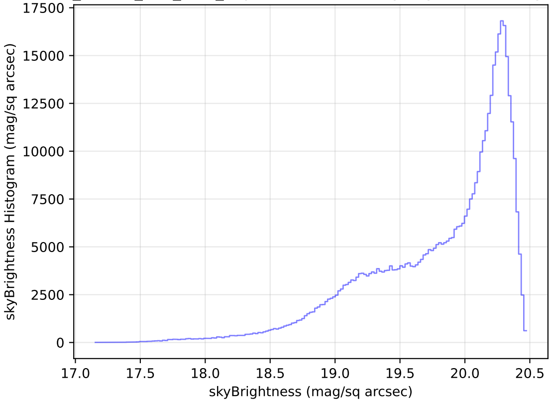
ddf_loaded_fl15_v3.4_10yrs WFD i band: skyBrightness Histogram
