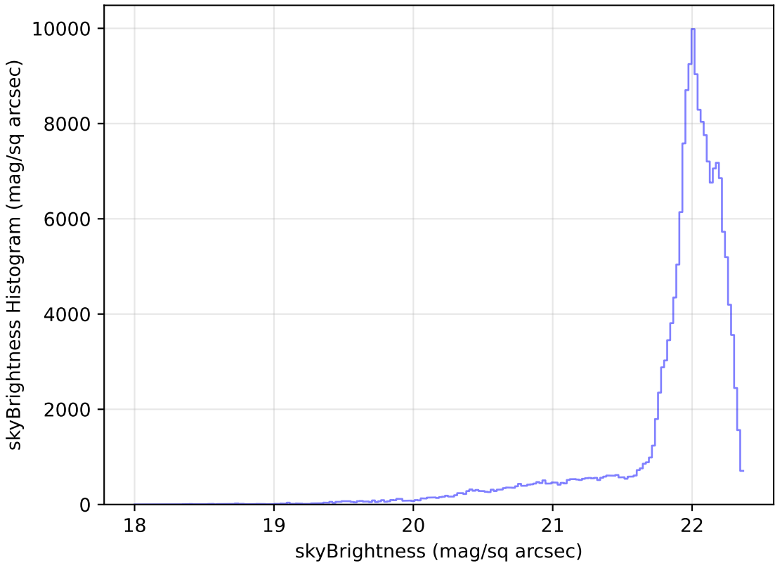
ddf_loaded_fl15_v3.4_10yrs WFD g band: skyBrightness Histogram
