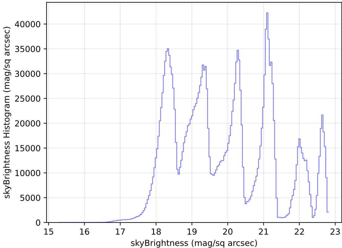
ddf_loaded_fl15_v3.4_10yrs WFD all bands: skyBrightness Histogram
