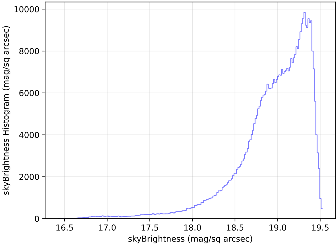
ddf_loaded_fl15_v3.4_10yrs All sky z band: skyBrightness Histogram
