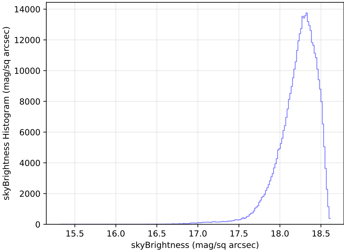
ddf_loaded_fl15_v3.4_10yrs All sky y band: skyBrightness Histogram
