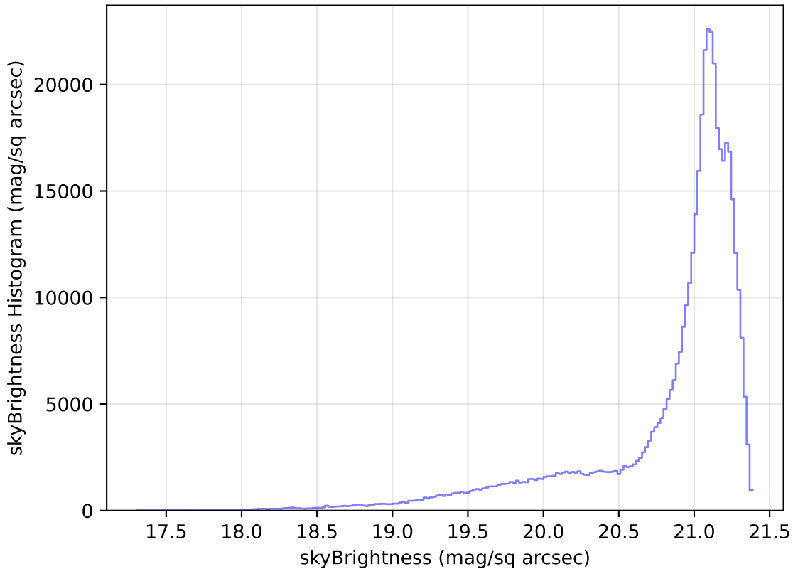
ddf_loaded_fl15_v3.4_10yrs All sky r band: skyBrightness Histogram
