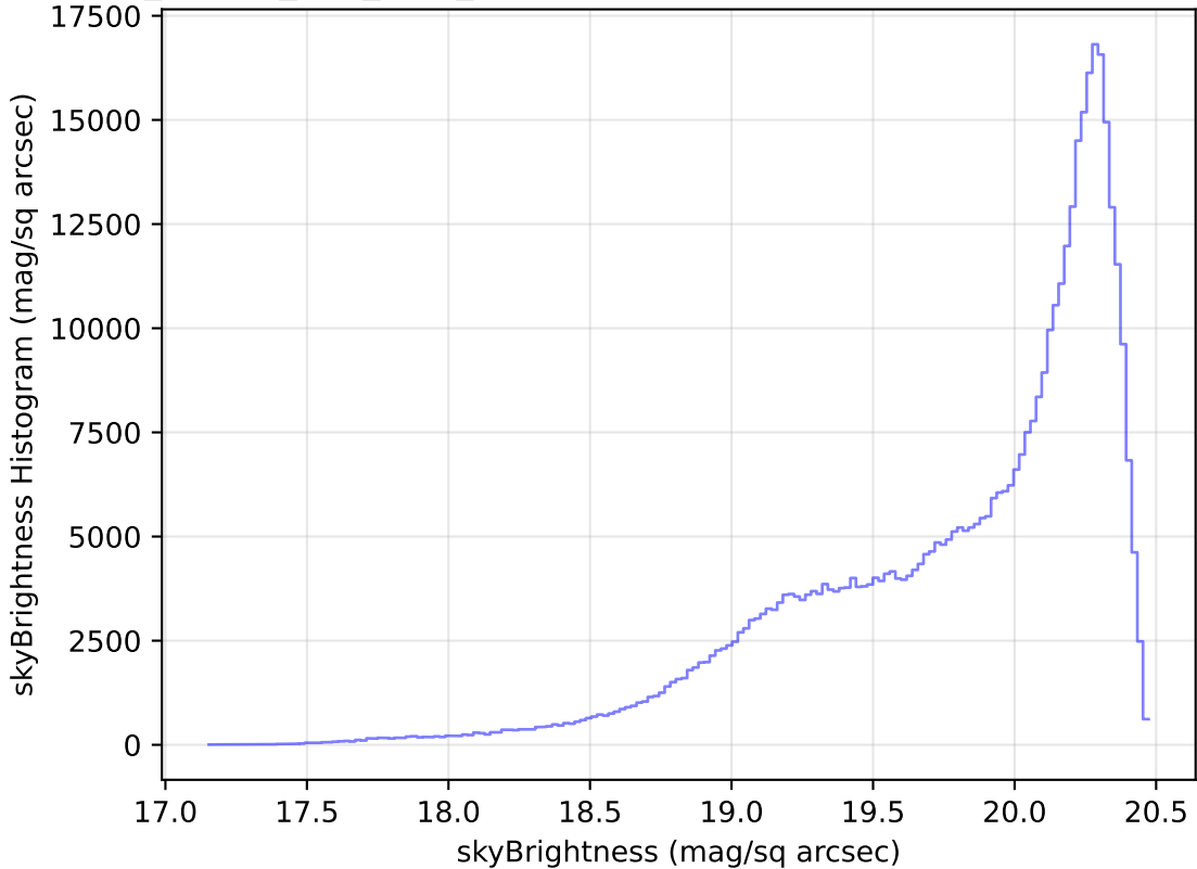
ddf_loaded_fl15_v3.4_10yrs All sky i band: skyBrightness Histogram
