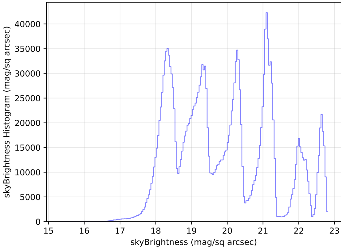
ddf_loaded_fl15_v3.4_10yrs All sky all bands: skyBrightness Histogram
