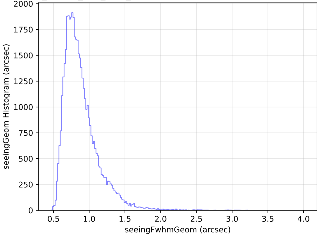
ddf_loaded_fl15_v3.4_10yrs Yr 1 z band: seeingGeom Histogram
