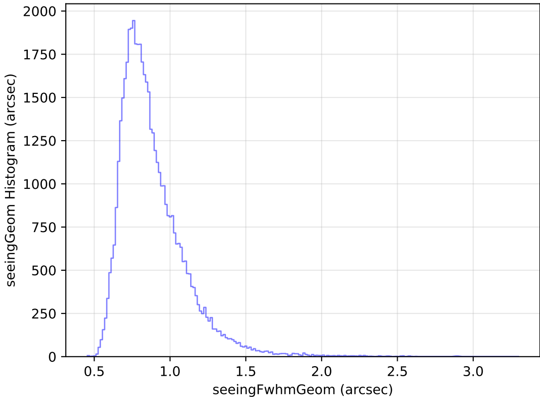
ddf_loaded_fl15_v3.4_10yrs Yr 1 y band: seeingGeom Histogram
