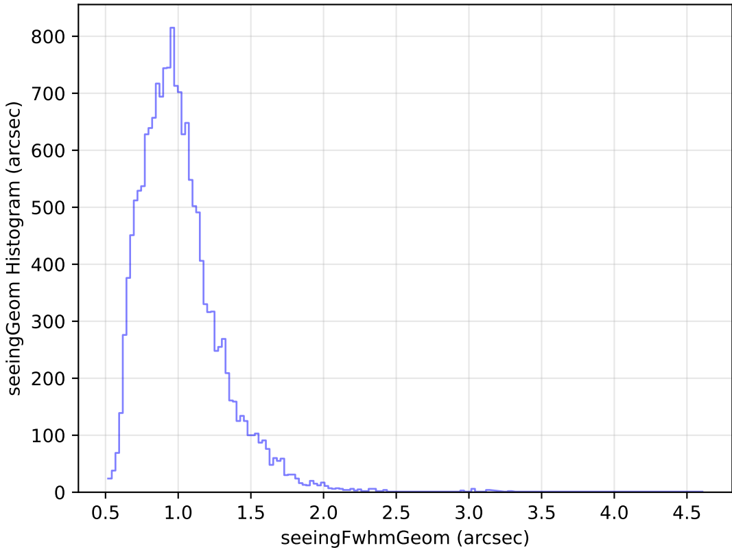
ddf_loaded_fl15_v3.4_10yrs Yr 1 u band: seeingGeom Histogram
