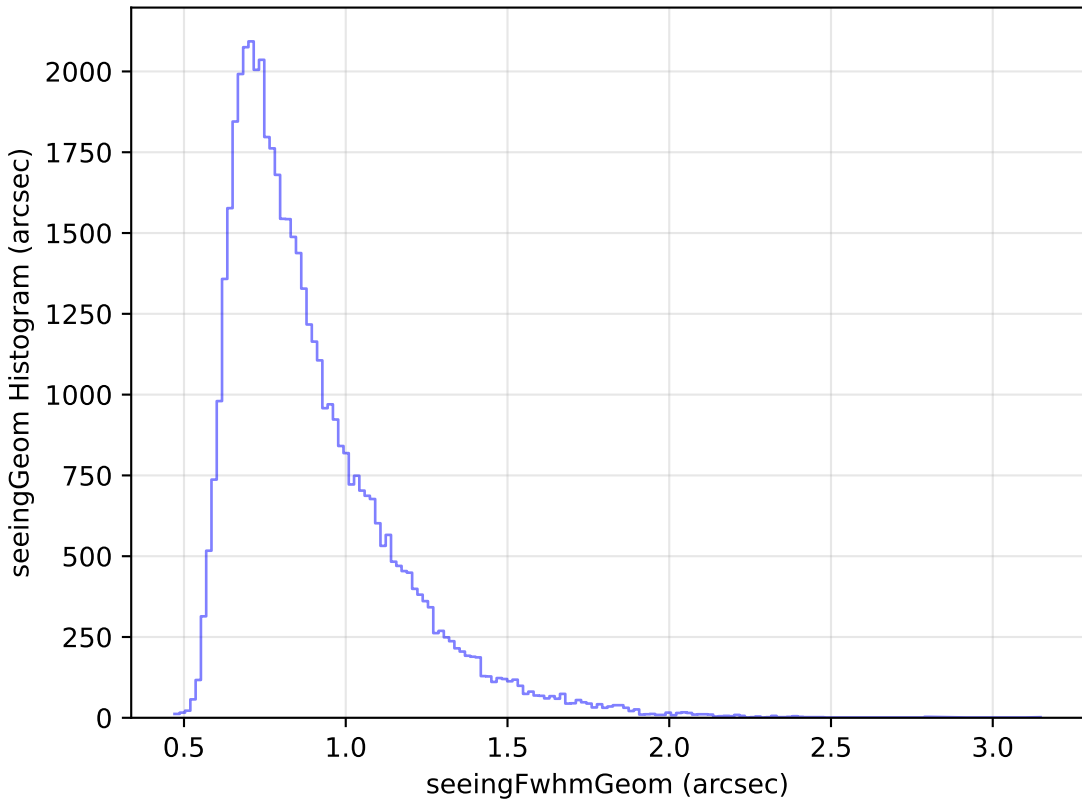
ddf_loaded_fl15_v3.4_10yrs Yr 1 r band: seeingGeom Histogram
