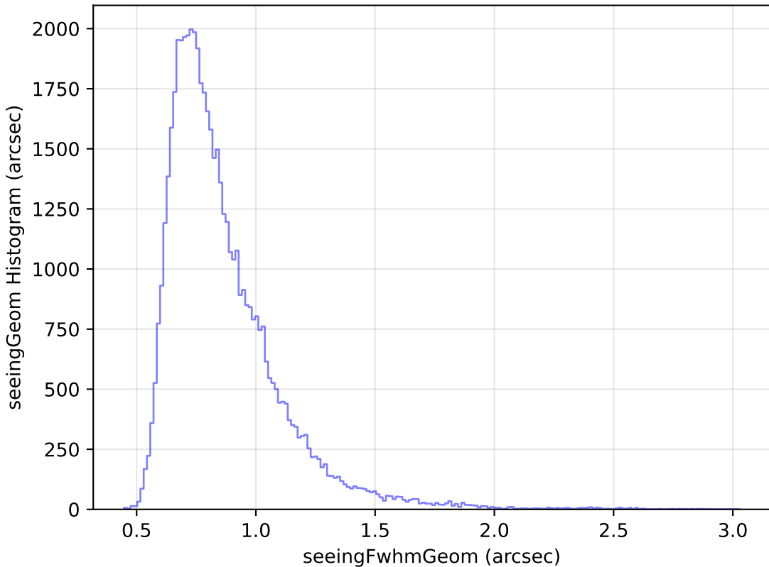
ddf_loaded_fl15_v3.4_10yrs Yr 1 i band: seeingGeom Histogram
