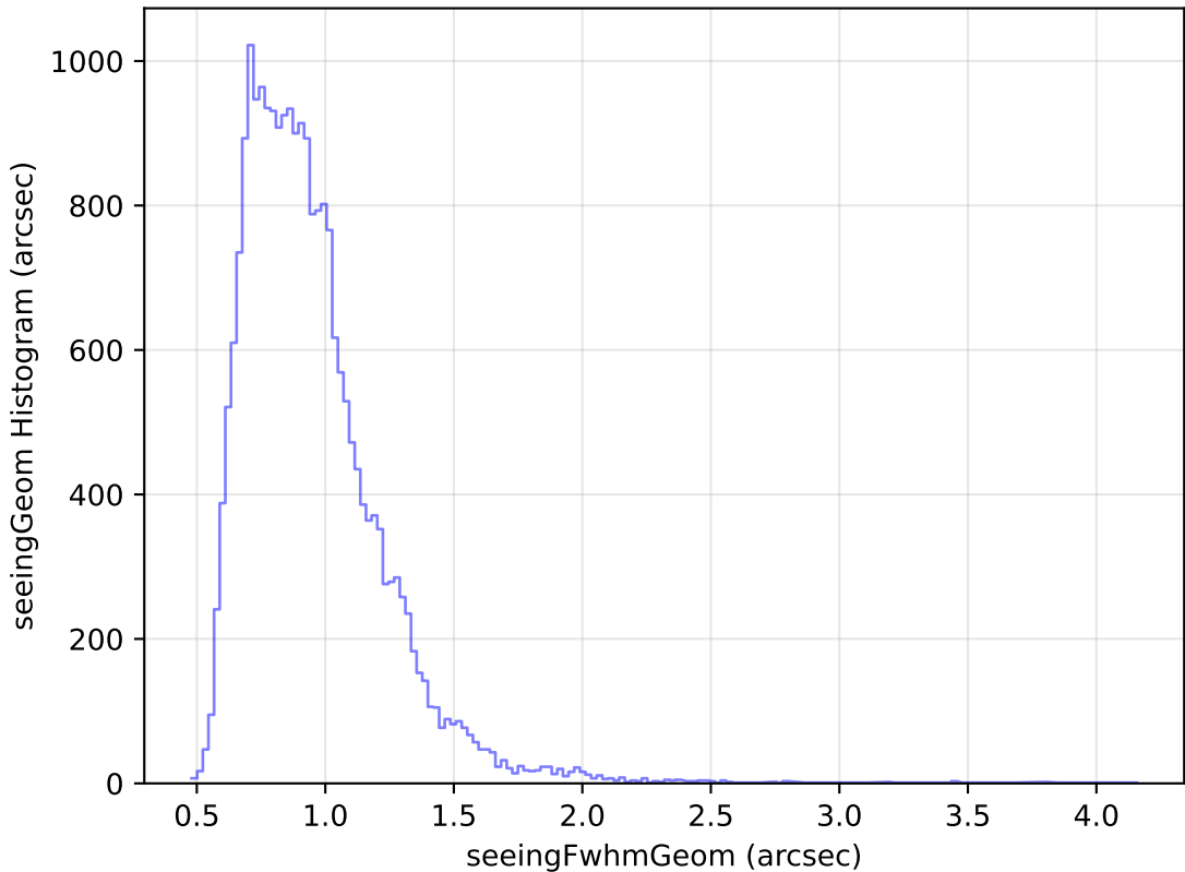
ddf_loaded_fl15_v3.4_10yrs Yr 1 g band: seeingGeom Histogram
