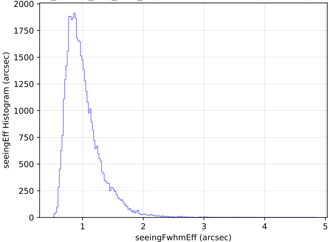
ddf_loaded_fl15_v3.4_10yrs Yr 1 z band: seeingEff Histogram
