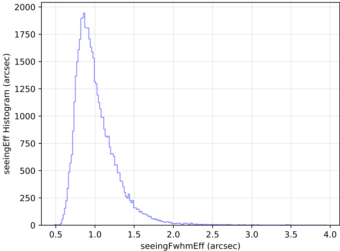
ddf_loaded_fl15_v3.4_10yrs Yr 1 y band: seeingEff Histogram
