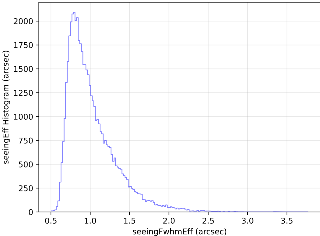
ddf_loaded_fl15_v3.4_10yrs Yr 1 r band: seeingEff Histogram
