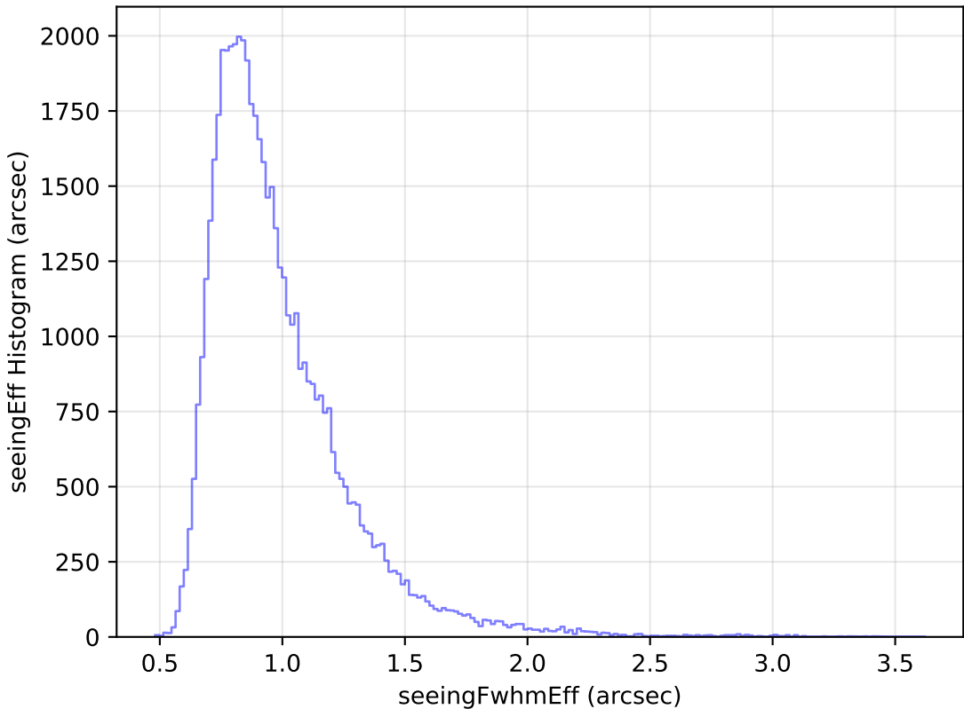
ddf_loaded_fl15_v3.4_10yrs Yr 1 i band: seeingEff Histogram
