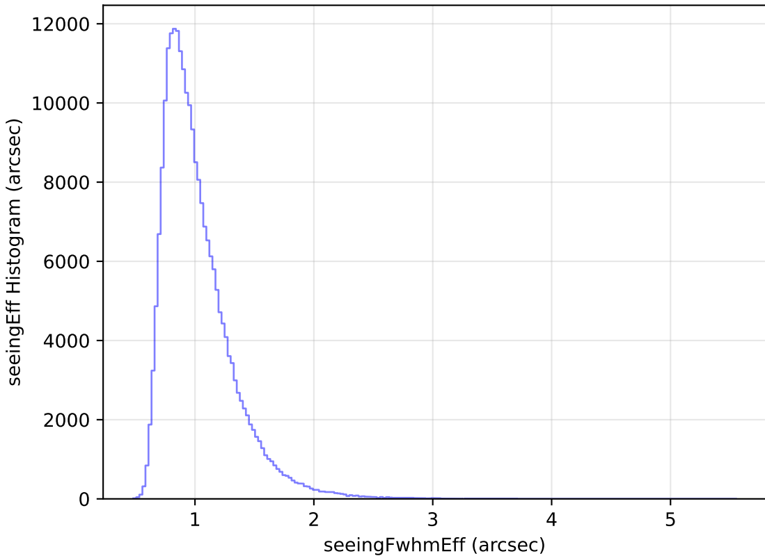
ddf_loaded_fl15_v3.4_10yrs Yr 1 all bands: seeingEff Histogram
