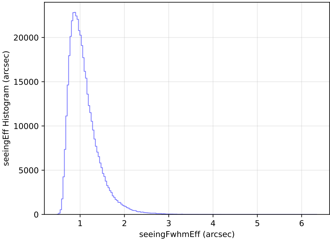
ddf_loaded_fl15_v3.4_10yrs WFD z band: seeingEff Histogram
