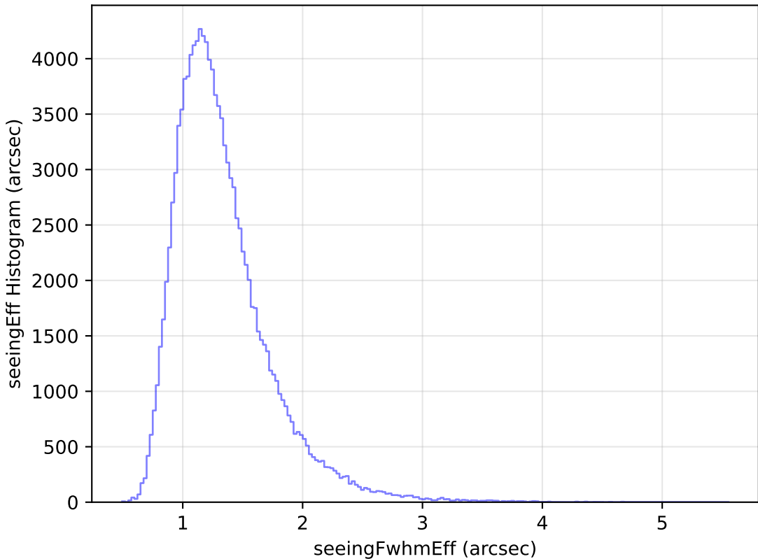
ddf_loaded_fl15_v3.4_10yrs WFD u band: seeingEff Histogram
