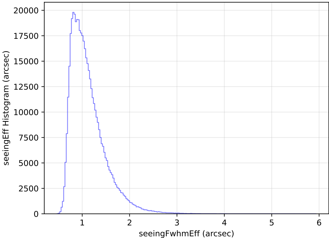
ddf_loaded_fl15_v3.4_10yrs WFD r band: seeingEff Histogram
